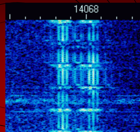
PACTOR Trace
